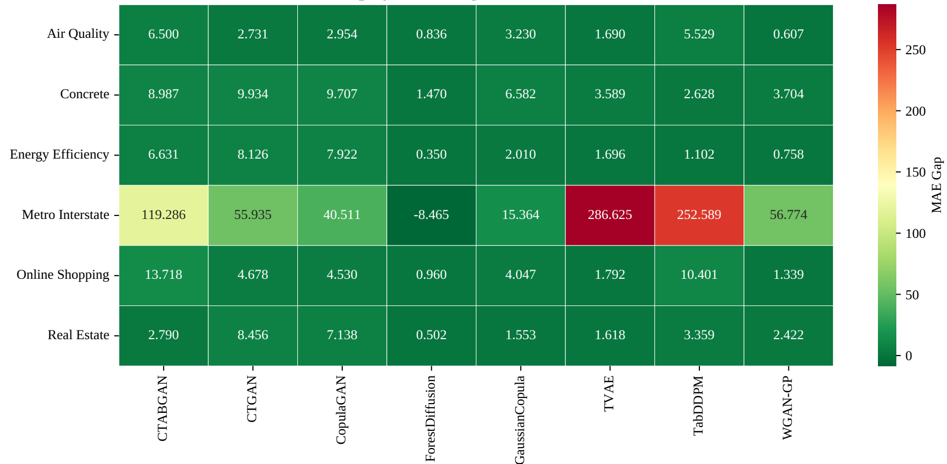
MAE Gap by dataset × generator (10-seed mean)
